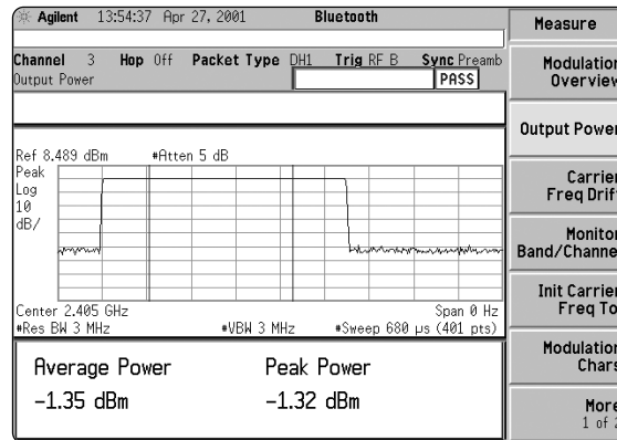
Figure 3. Output power measurement under measure menu.
