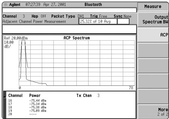
Figure 14. ACP measurement with spectrum display.
