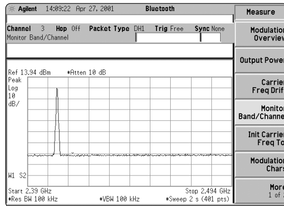
Figure 9. Monitor/band channel measurement under measure menu. The input signal stays at one channel.
