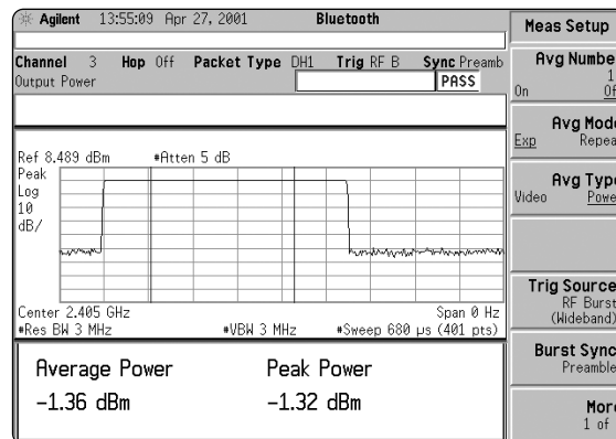
Figure 4. Measurement setup menu for output power.
