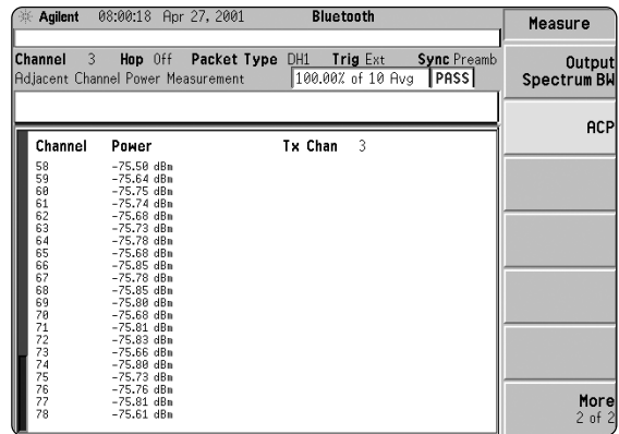
Figure 15. Zoom in on the numeric summary table for the ACP measurement. Notice a scroll bar at the left of the display window. Users can scroll up or down to view the channels of interest by pressing [↑] or [↓] hardkeys or by turning the knob.
