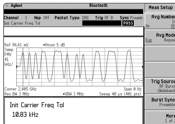
Figure 6. Measurement setup menu for initial carrier frequency tolerance.
