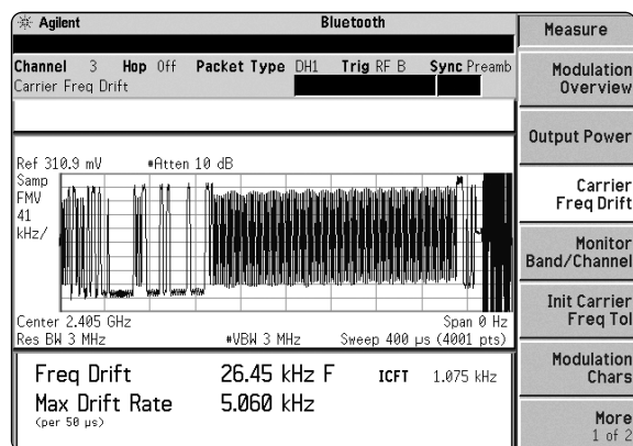
Figure 7. Carrier frequency drift measurement under measure menu
