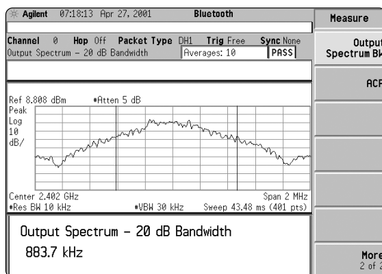
Figure 12. 20 dB bandwidth measurement is under measure menu (output spectrum BW).
