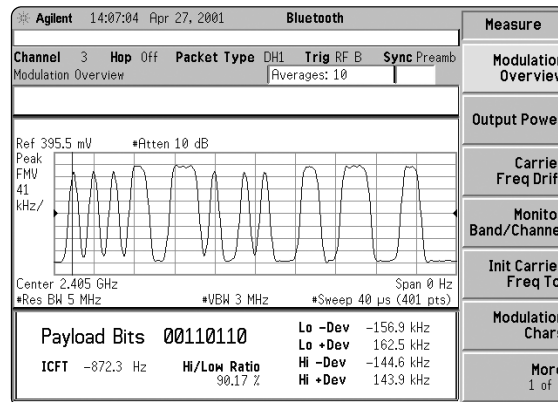
Figure 11. Modulation overview measurement is under measure menu.
