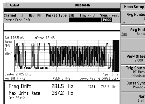
Figure 8. Measurement setup menu for carrier frequency drift.
