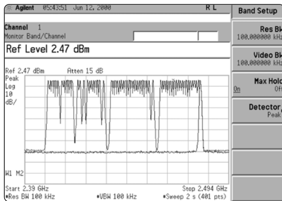
Figure 10. Measurement setup menu for monitor/band channel. The input signal is hopping across Bluetooth RF band.
