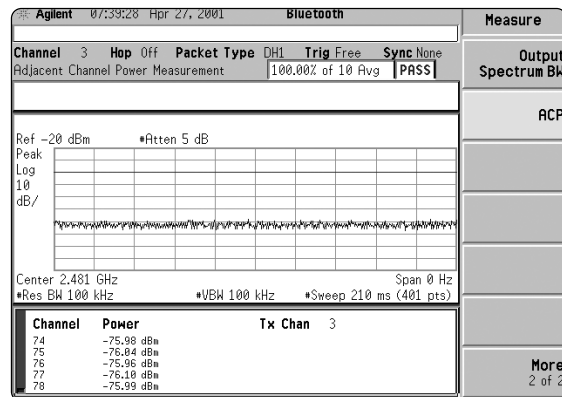
Figure 13. ACP measurement is under measure menu.
